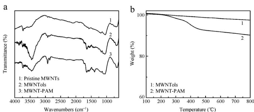
Fig. 8. (a) FT-IR spectral profile of pristine MWNTs, MWNTols, and MWNT-PAM and (b) TGA curves of MWNTols and MWNT-PAM.
