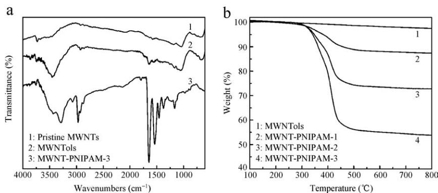
Fig. 5. (a) FT-IR spectral profile of pristine MWNTs, MWNTs, and MWNT-PNIPAM-3; (b) TGA curves of MWNTs, MWNT-PNIPAM-1, MWNT-PNIPAM-2, and MWNT-PNIPAM-3.
